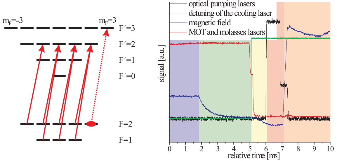
Figure 3.21: Transfer from the MOT into the quadrupole trap. Left figure: Illustration of the optical pumping scheme. Lasers resonant to the F = 2 \rightarrow F' = 2 and F = 1 \rightarrow F' = 2 transitions are used. The pumping collects the atoms in the |2, 2\rangle ground state (marked with the red ellipse), which does not couple to the \sigma^+ polarized laser beams. Right figure: Stages of the transfer into the magnetic trap, as described in the text. Blue — compressed MOT. Green — optical molasses. Yellow — delay time for tuning the optical pumping laser. Red — optical pumping. Orange — capture of the atoms in the magnetic trap. Further details in the text.
