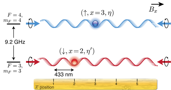
FIG. 1. Transport of single Cs atoms in state-dependent periodic potentials. Two independent optical lattices originate from standing waves of opposite circular polarization but identical wavelength \lambda = 866\ \text{nm} . Depending on the internal state, \uparrow or \downarrow , atoms experience one or the other lattice potential. An optoelectronic servo-lock loop allows the position of each lattice to be arbitrarily controlled. The atom’s position is retrieved with single-site resolution by fluorescence imaging. The parameter \eta accounts for other degrees of freedom, such as the atom’s position perpendicular to the lattice or, in general, other hidden physical aspects. The quantization axis is defined by the small bias magnetic field B_x , which is chosen along the two optical lattices. F and m_F denote, respectively, the total angular momentum and its projection along the quantization axis for both internal hyperfine states.
