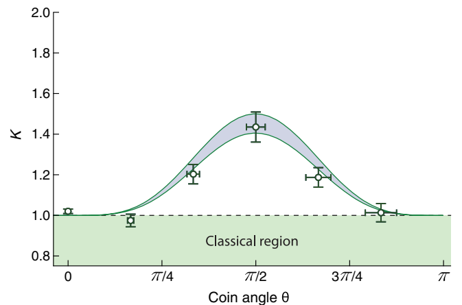
FIG. 4. Leggett-Garg correlation measurement witnessing the degree of quantumness. Maximum violation occurs for a fair coin ( \theta = \pi/2 ), while no violation occurs for classical transport at \theta = 0 and \theta = \pi . The solid line is the theoretical prediction based on quantum mechanics of the LG correlation function K for a decoherence-free quantum walk (upper curve) and for a quantum walk with 10% decoherence per step (lower curve). The vertical error bars represent 1\sigma uncertainty, while the horizontal error bars denote a systematic uncertainty on the coin angle.
