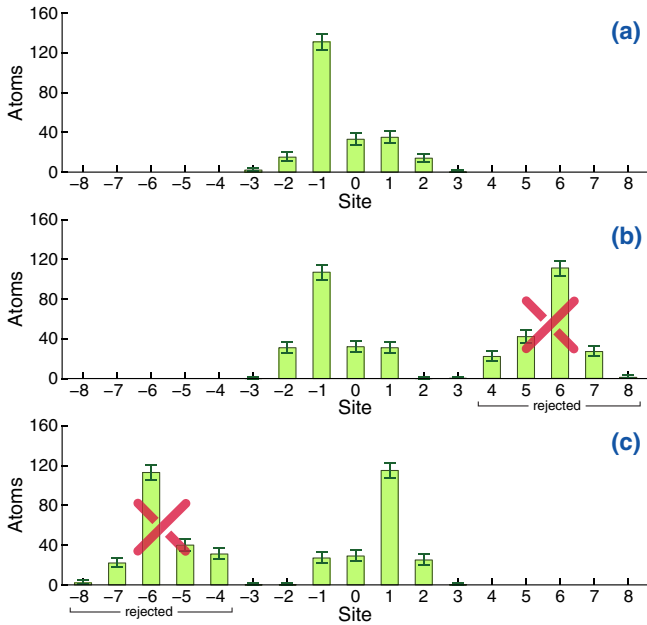
FIG. 3. Violation of Leggett-Garg inequality probing a four-step quantum walk. The spatial distribution of single atoms is reconstructed by measuring their positions at time t_3 : (a) If we do not observe which trajectory the atom has taken at t_2 , the distribution exhibits a pronounced peak on the left-hand side. However, when we conclude from an ideal negative result whether the atom at time t_2 was in (b) x = -1 or (c) x = 1 , we obtain two distributions that resemble the mirror image of one other. The events in which the atom’s position has been affected by Q(t_2) measurement are recognized through the larger displacement and, thus, rejected. Because the overall number of probed atoms, 404, is the same in (b) and (c), the retained events can be added together to produce the position distribution at t_3 conditioned on having measured the position at t_2 . The sum distribution (not shown) is symmetric and differs strongly from the asymmetric distribution in (a). The vertical error bars represent 68% Clopper-Pearson confidence intervals.
