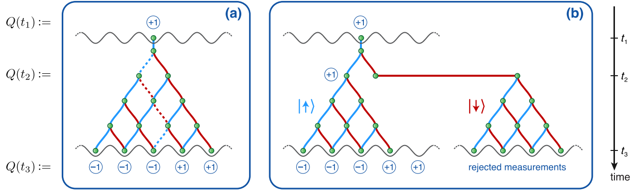
FIG. 2. Ideal negative measurements test the nonclassicality of quantum walks. (a) Schematic representation of a four-step quantum walk containing 16 possible trajectories, which according to quantum mechanics, the Cs atom simultaneously follows. Conversely, upholders of realism believe that in each experiment the atom follows a definite trajectory connecting the initial and final point, e.g., the dashed line shown in the figure. The outcomes \pm 1 of Q(t_i) measurements are indicated with circles, where Q(t_1) is identified with the initial-state preparation, whereas Q(t_2) and Q(t_3) are related to position measurements. For instance, measurements at times t_1 and t_3 yield the correlation function \langle Q(t_3)Q(t_1) \rangle . (b) To measure the correlation function \langle Q(t_3)Q(t_2) \rangle , we use at time t_2 an ideal negative measurement scheme, which ensures the noninvasiveness of Q(t_2) : On the condition that only atoms in the \downarrow state are transported at t_2 far away to the right, atoms in \uparrow continue their walk undisturbed. In case Q(t_2) measurement has not removed the atom, measuring at t_3 the atom's position yields Q(t_3) conditioned to the state (\uparrow, x = -1) at t_2 . Likewise, we obtain Q(t_3) conditioned to (\downarrow, x = +1) by transporting at t_2 the atom in \downarrow far away to the left (not shown in the figure).
