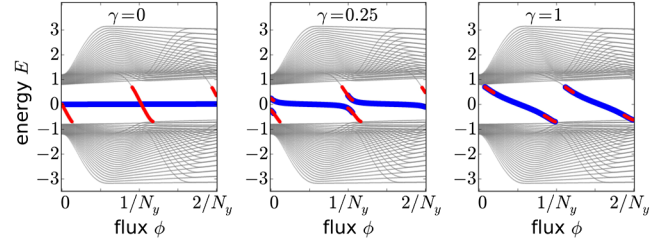
FIG. 3. Spectra of the Qi-Wu-Zhang model as a function of the magnetic flux (two cycles shown), computed on a lattice of finite width (36 sites) along y and for a fixed quasimomentum ( k_x = 0 ). \gamma indicates the hopping amplitude at the edge ( \gamma = 0 for open and \gamma = 1 for periodic boundary conditions). States with more than 30% weight in the first two rows at the top (bottom) edge are marked by thick red (blue) lines.
