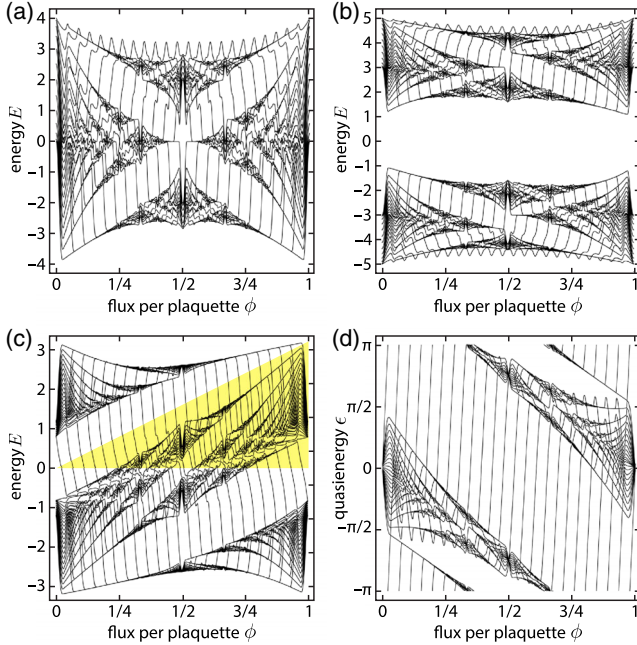
FIG. 2. Examples of Hofstadter spectra analogous to those shown in Fig. 1, but computed for a lattice of finite width ( 24 sites with periodic boundary conditions), and still infinite along x . For better visibility of the spectral flow, the spectra are shown for a given quasimomentum only ( k_x = 0 ).
