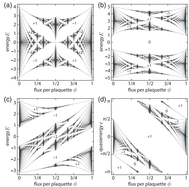
FIG. 1. Examples of Hofstadter butterfly spectra for (a) a simple charged particle on an infinite square lattice (Harper model), (b) a topologically trivial multiband insulator (Qi-Wu-Zhang model with u = 3 of Ref. [16]), (c) a topological multiband insulator (same Qi-Wu-Zhang model with u = -1.2 ), and (d) a topological Floquet insulator [Rudner model of Ref. [17] with \delta_{AB} = 0 and JT/5 chosen for the first four segments as (3/8, 3/8, 5/8, 5/8)\pi ]. The topological indices of a few representative band gaps are shown in the figure.
