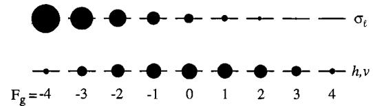
Fig. 6. Ground-state population after decay of an initially isotropic excited state distribution with \langle m \rangle = 0 by emitting a circular polarized photon \sigma_l (upper part). The dot sizes correspond to the individual populations of the sublevels. For comparison, the situation is completely different for the h,v -correlation: detecting a linearly h - or v -polarized photon (lower part) does not lead to any orientation of the atom. Therefore, any succeeding excitation will result in almost equal probabilities for detecting a h - or a v -polarized photon in the next spontaneous emission, leading to g_{hv}^{(2)}(\tau = 0) \approx 1 .
