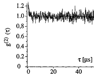
Fig. 4. Total intensity-intensity correlation function g^{(2)}(\tau) of a single-atom fluorescence in the MOT 00 field ( \delta = -1.1\Gamma , I = 1.3 I_0 , integration time 10.4 min). Solid line: exponential fit.
