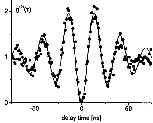
Fig. 1. Intensity–intensity correlations in the resonance fluorescence of a single Cs atom stored in a MOT. The uncorrelated background of stray-light photons has been measured independently and subtracted. Details can be found in [9] and [10].
