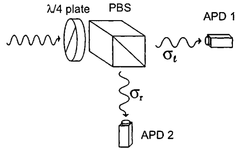
Fig. 2. Optics for polarization-resolved photon correlations. To measure correlations between right- and left-handed \ell/r (“circular correlations”), a quarter wave plate is placed before the polarizing beam splitter (PBS). For vertical and horizontal v/h (“linear correlations”) components only, a polarizing beam splitter is used. For total intensity-intensity correlations, the fluorescence is divided by a nonpolarizing beam splitter.
