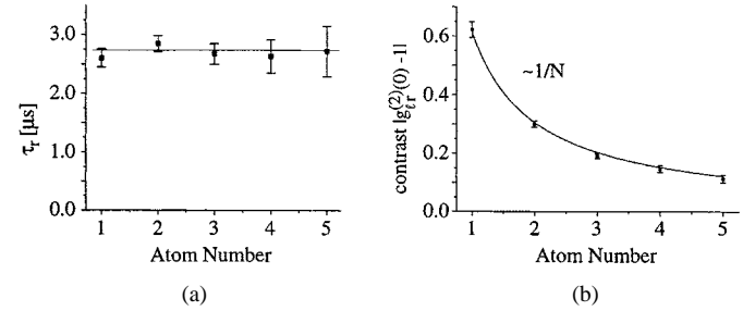
Fig. 5. Measured characteristic (a) relaxation time and (b) contrast of the cross correlations for circular polarization components as a function of the number of observed atoms recorded at constant trap parameters.
