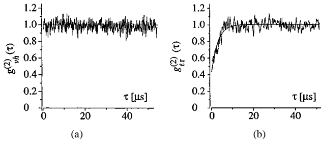
Fig. 3. Measured photon correlations from a single atom in the MOT 00 field. (a) Correlation function g_{vh}^{(2)}(\tau) for orthogonal linear polarization components ( \delta = -1.8\Gamma , I = 0.95 I_0 , integration time 6.3 min). (b) Correlation function g_{lr}^{(2)}(\tau) for orthogonal circular polarization components ( \delta = -2.7\Gamma , I = 0.7 I_0 , integration time 11.1 min). Solid line: exponential fit.
