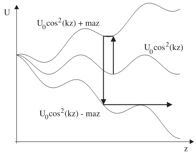
FIGURE 8 Standing wave potential shown in reference frames accelerated with +a, 0, -a , respectively. Here the worst case of maximal energy gain at a = 0.42a_{\text{max}} is illustrated: due to the abrupt changes of the accelerating potential an initially motionless atom can gain enough energy to leave the trap
