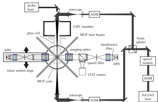
FIGURE 1 Scheme of the experimental setup. The fixed imaging optics on the right-hand side is used to monitor the fluorescence at the MOT position. The imaging optics mounted on the linear-motion stage on the left-hand side is used for atom detection at any spot along the dipole trap
