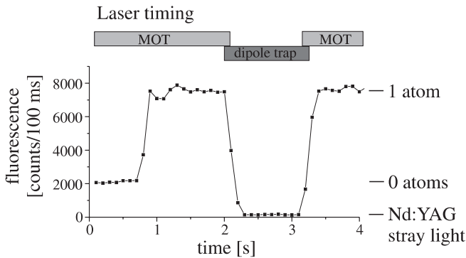
FIGURE 2 Storage of a single atom in the dipole trap for 1 s. The fluorescence signal of the atom demonstrates the trapping in the dipole trap and recapturing by the MOT
