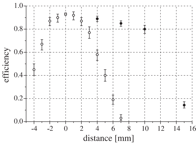
FIGURE 4 Transportation efficiency of the optical conveyor belt for a constant acceleration of 500 \text{ m/s}^2 . Each data point results from \sim 100 shots performed with one atom each. Empty circles : the atom is detected by resonant illumination at its new position. Filled circles : more efficient detection by moving the atom back and recapturing it in the MOT
