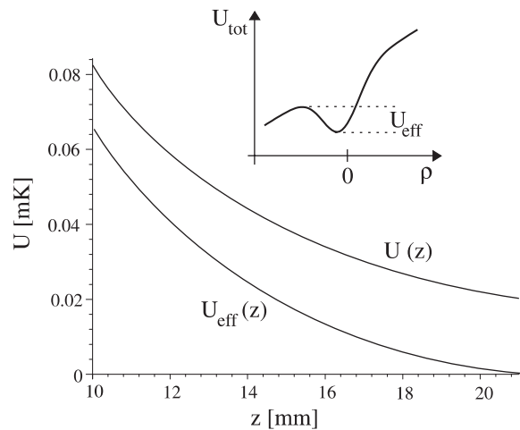
FIGURE 5 Reduction of the trap depth due to gravity. The inset shows the sum U_{\text{tot}} of the dipole potential and the gravitational potential versus the radial coordinate \varrho for an arbitrary potential well along the optical z -axis. Below, the resulting effective potential depth U_{\text{eff}}(z) is compared to the pure dipole potential U(z) for z = 10\text{--}21 \text{ mm} . The position z = 21 \text{ mm} , where U_{\text{eff}} completely disappears, represents the fundamental upper bound for the transportation distance in our dipole trap
