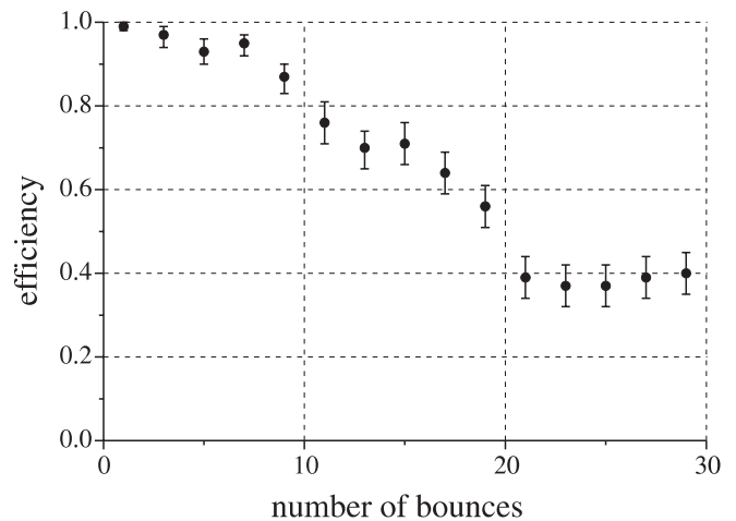
FIGURE 6 ‘Single-atom shuttle’. The measured efficiency is plotted versus the number of bounces, with a displacement distance of 1 mm each and with an acceleration of 5000 \text{ m/s}^2
