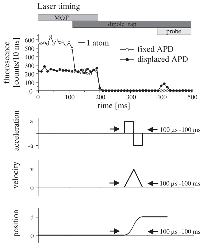
FIGURE 3 Single-atom conveyor belt. The fluorescence signal of the atom is recorded by both APDs during the transportation sequence. The fixed APD initially confirms the presence of the atom in the MOT. During transfer into the dipole trap the MOT fluorescence is decreased due to the light shift. Initially, the displaced APD (filled circles) does not see the trapped atom but only detects stray light of the MOT laser beams. The burst of fluorescence at t = 400 \text{ ms} originates from the same atom displaced by 1 mm, which is illuminated in the dipole trap with a resonant probe laser
