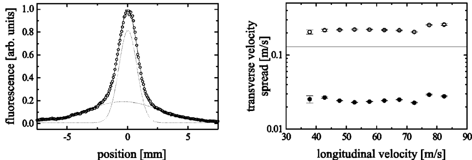
FIG. 11. Measurement of the transverse velocity spread of the atomic beam. (a) CCD fluorescence profile (open circles) fitted with the sum (solid line) of two Gaussian profiles (dashed lines). (b) Transverse velocity spread deduced from the two Gaussian profile components as a function of the longitudinal velocity. The horizontal line corresponds to the Doppler velocity limit for cesium atoms.
