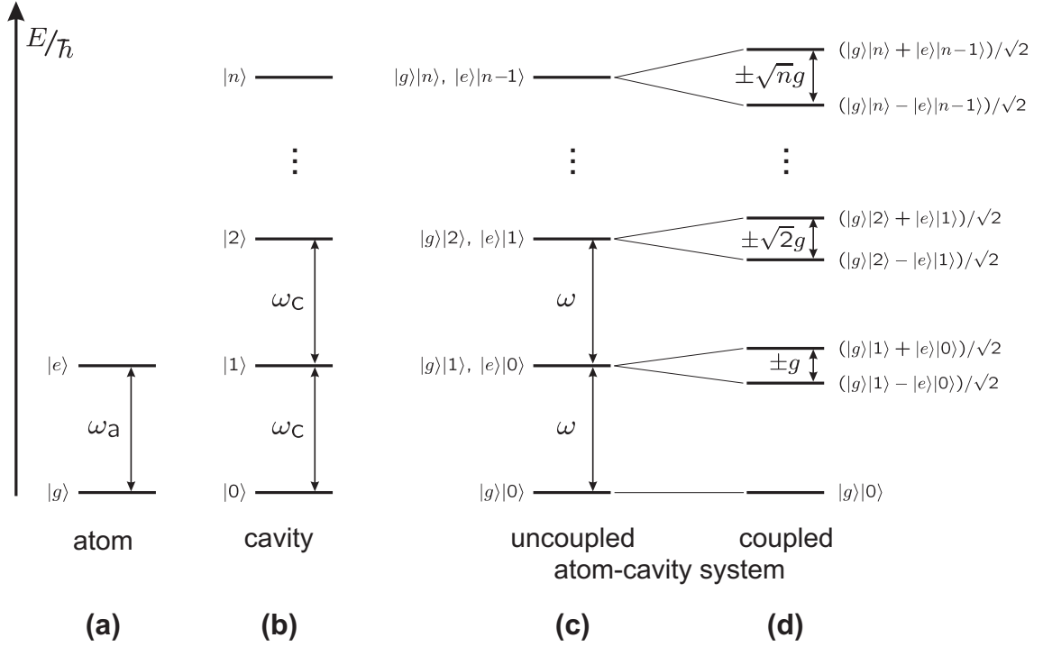
Figure 4.1: Eigenstates of the resonant atom-cavity system. For the resonant system, the frequency spacing \omega coincides with \omega_a and \omega_c .
