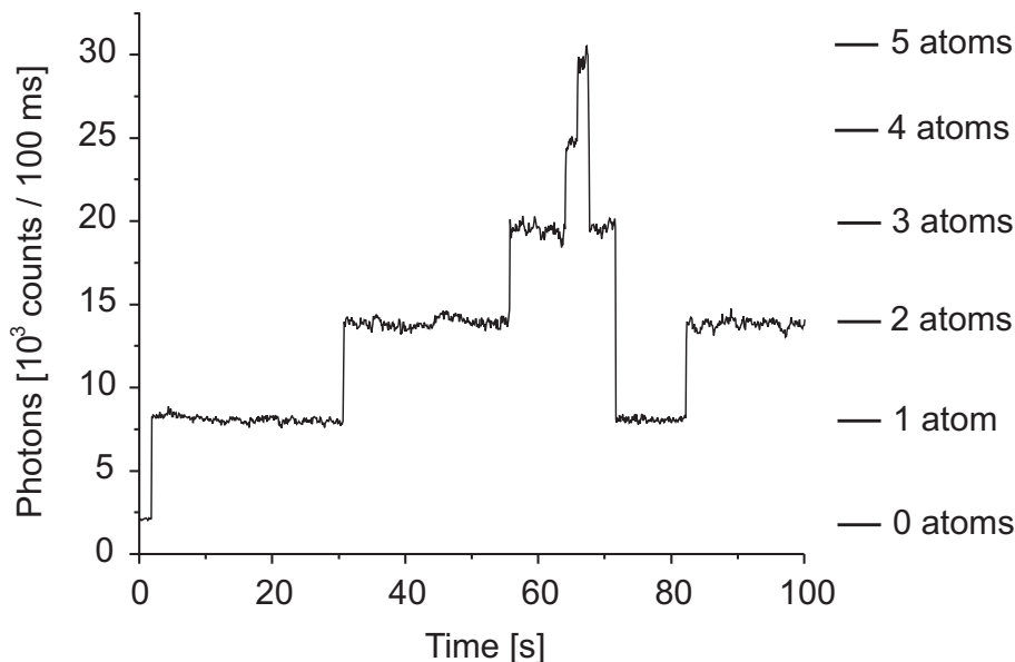
Figure 1.5: APD signal of the MOT fluorescence. Each trapped atom contributes the same amount of fluorescence to the signal, allowing us to determine their exact number. When an atom enters or leaves the trap, the count rate instantaneously increases or decreases accordingly.
