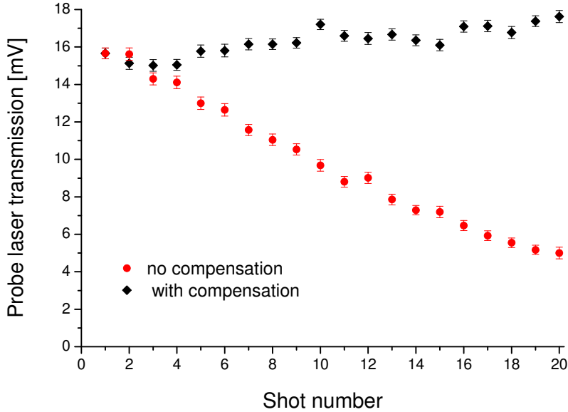
Figure 3.17: Probe transmission with (diamonds) and without (circles) compensation of the cavity thermal drifts. The transmission is measured for 20 successive experimental shots within one experimental run. The compensation method used is the center-of-mass method. A slight increase of the cavity transmission in (b) originates from a drift of the incident power of the probe laser.
