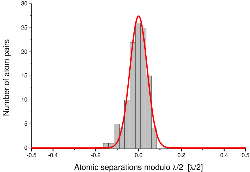
Figure 2.6: Histogram of the atomic separations averaged over more than 9 measurements each and calculated modulo \lambda/2 . The data analyzed are the one from Fig. 2.5.
