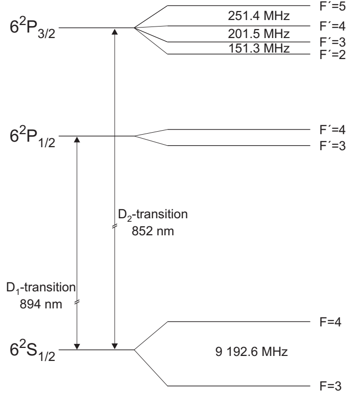
Figure A.1: Level scheme of the first excited states in ^{133}\text{Cs} .
